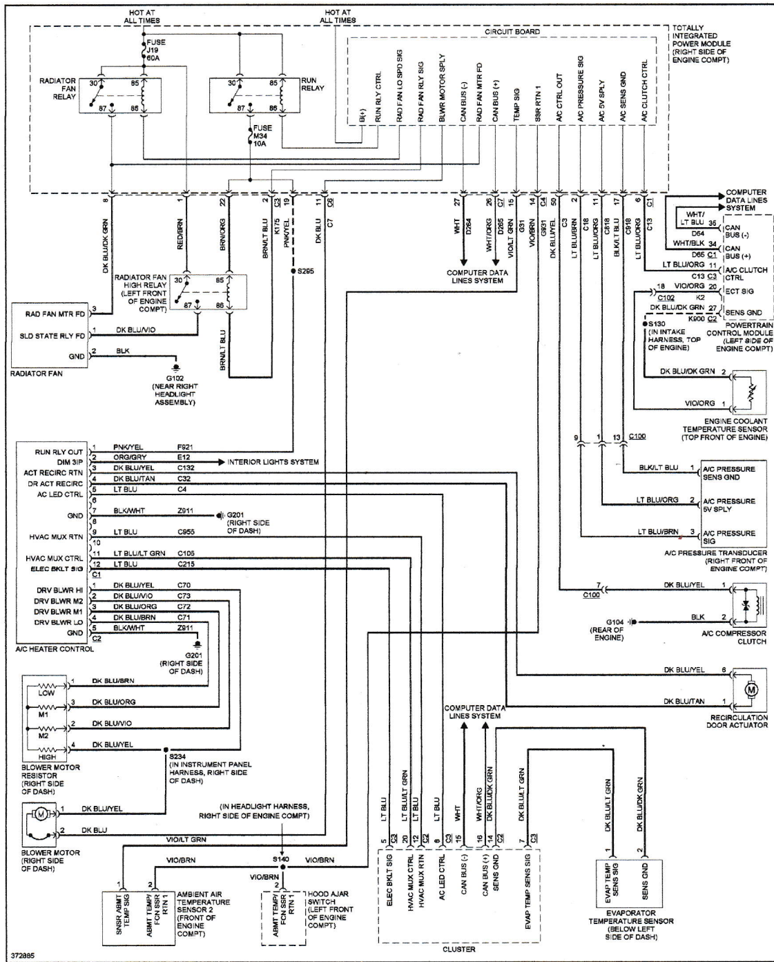
Fig. 2: Manual A/C Circuit
